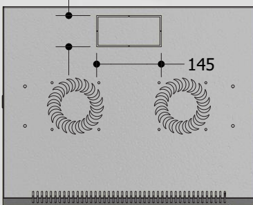
70 145 Top View
