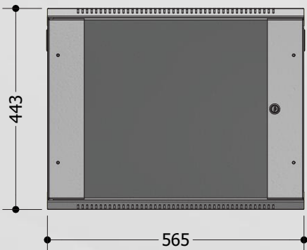
70 Front View
